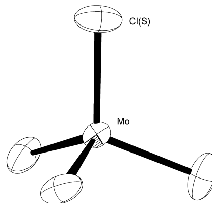
Figure 1. Structure of the complex anion of [PPh 4 ][MoClS 3 ] ( 2 ) with thermal ellipsoids at 50% probability level. Mo–S(Cl) 2.1727(1) Å.
