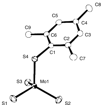
Figure 3. Structure of the complex anion of [\text{PPh}_4][\text{MoS}_3(\text{SMes})] ( 6c ) with thermal ellipsoids at 50% probability level.
