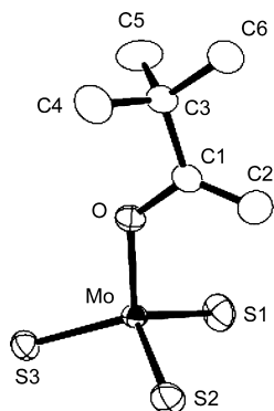
Figure 5. Structure of the complex anion of [\text{PPh}_4][\text{MoS}_3\{\text{OC}(\text{CH}_2)_2\text{tBu}\}] ( 8c ) with thermal ellipsoids at 50% probability level.
