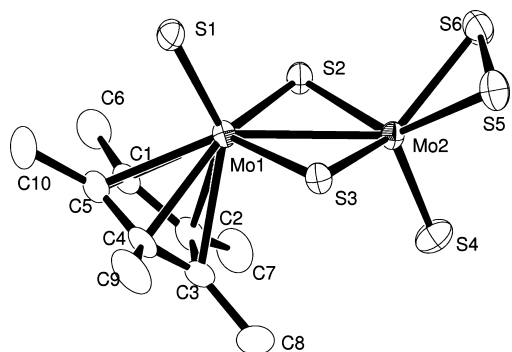
Figure 2. Structure of the complex anion of [\text{PPh}_4][\text{Cp}^*\text{Mo}(\text{S})(\mu\text{-S})_2\text{Mo}(\text{S})(\text{S}_2)] ( 5 ) with thermal ellipsoids at 50% probability level.
