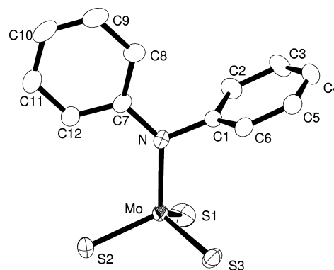
Figure 4. Structure of the complex anion of [\text{PPh}_4][\text{MoS}_3(\text{NPh}_2)] ( 7 ) with thermal ellipsoids at 50% probability level.
