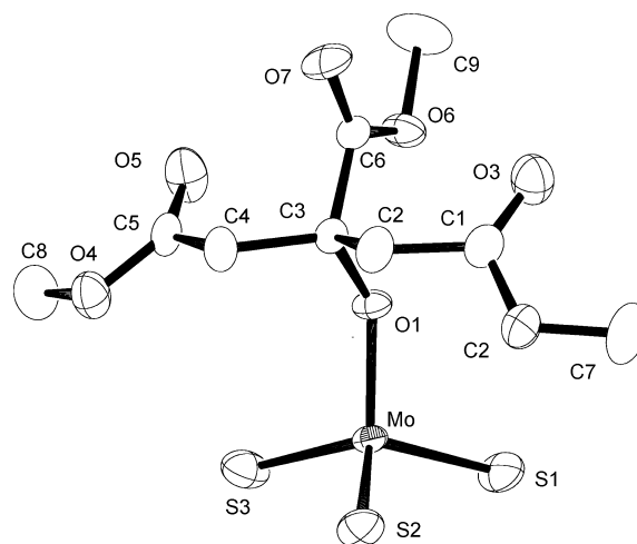
Figure 6. Structure of the complex anion of [\text{PPh}_4][\text{MoS}_3(\text{Me}_3\text{cit})] ( 9 ) with thermal ellipsoids at 50% probability level.
